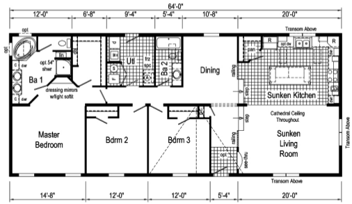
DE654-A 2864 Approx. 1749 Sq. Ft.
